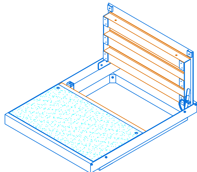
ISOMETRIC DETAIL
