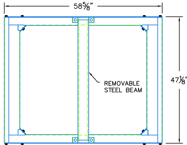
FRAME - PLAN VIEW
