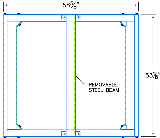
FRAME - PLAN VIEW
