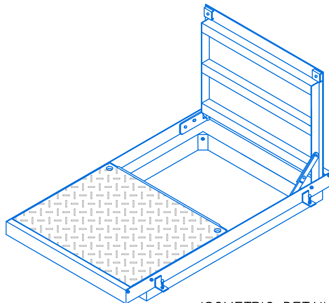
ISOMETRIC DETAIL
