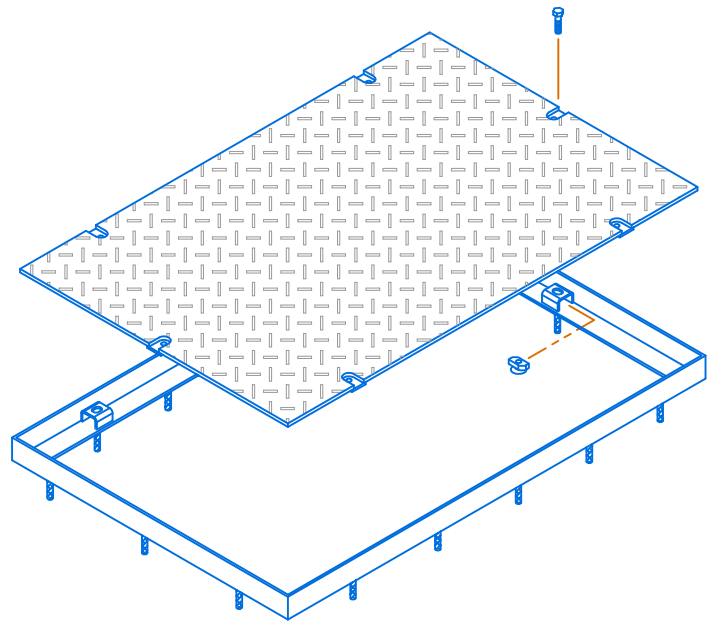
ISOMETRIC DETAIL
