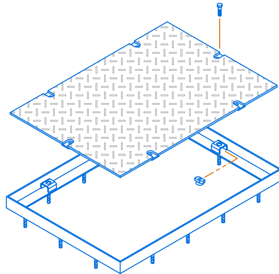
ISOMETRIC DETAIL
