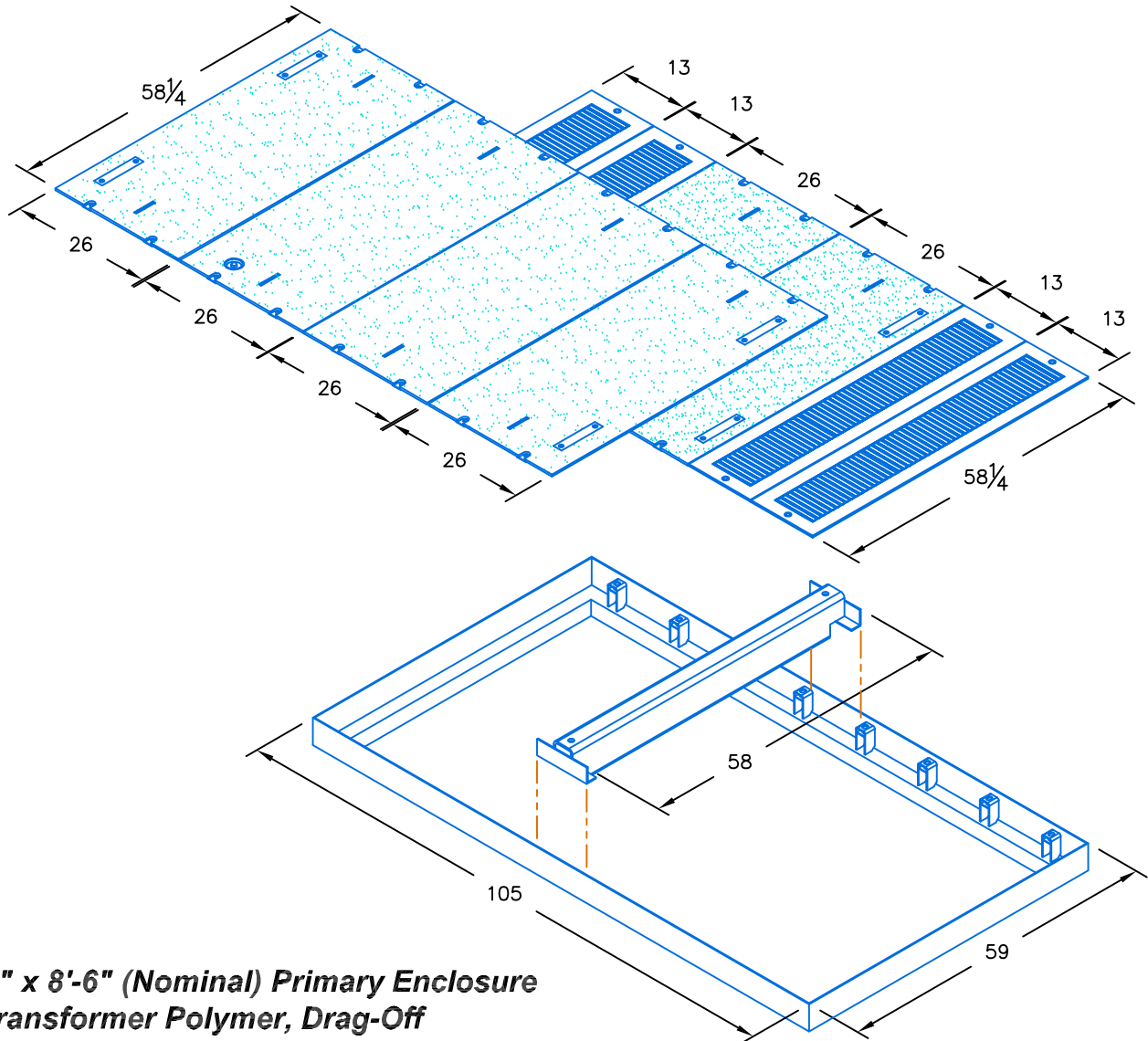
ISOMETRIC DETAIL
