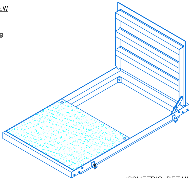
ISOMETRIC DETAIL
