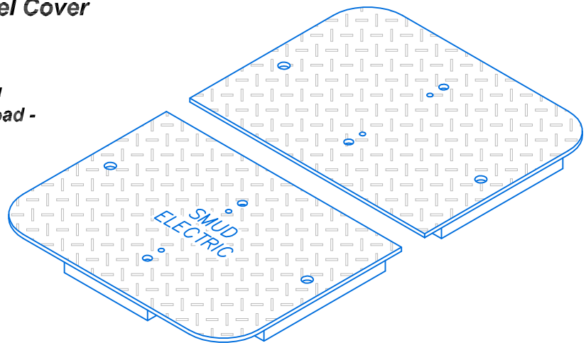
ISOMETRIC DETAIL
