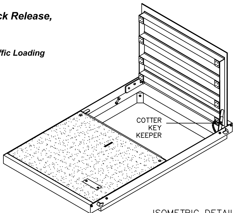
ISOMETRIC DETAIL
